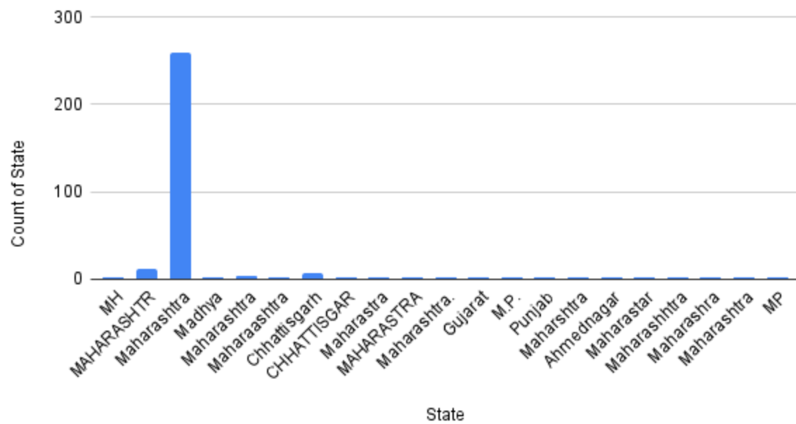
Count of State
