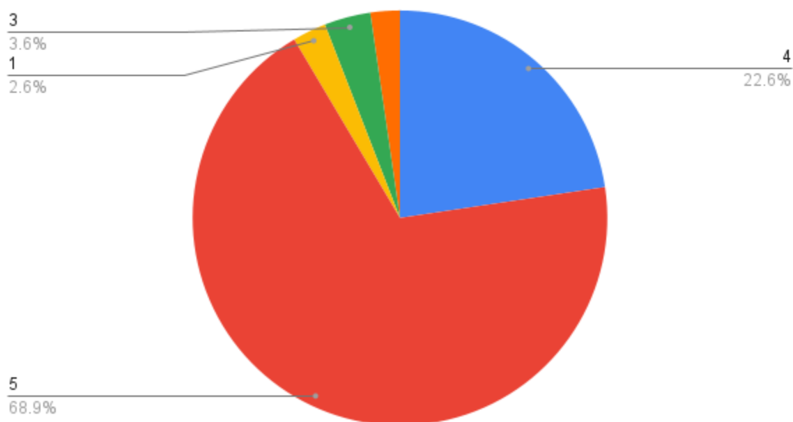
Count of How would you rate the Speakers?
