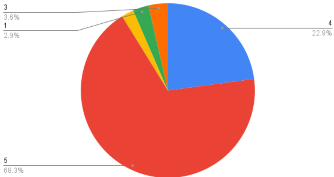
Count of How would you rate the overall webinar experience?
