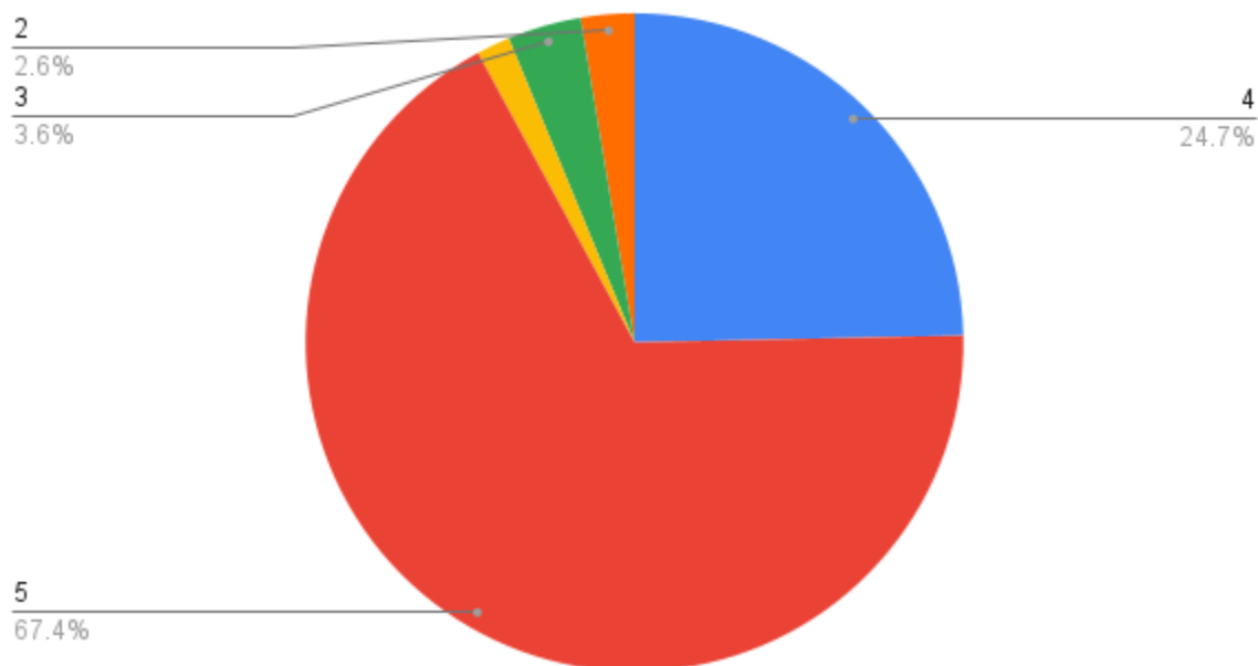
Count of How would you rate the content of the webinar?
